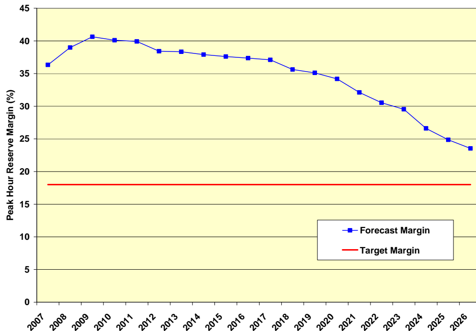
Figure 12: Forecast Pacific Northwest Annual Peak-hour Capacity Reserve Margin
