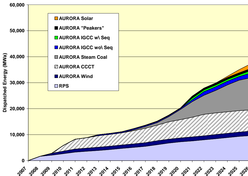
Figure 9: Forecast WECC incremental resource mix based on dispatched energy
