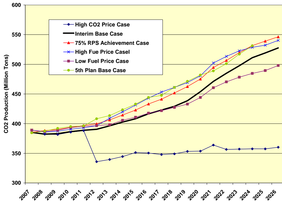
Figure 14: Interim base case and sensitivity case CO 2 production forecasts (WECC) (Note: scale of left axis begins at 300 million tons of CO 2 production)
