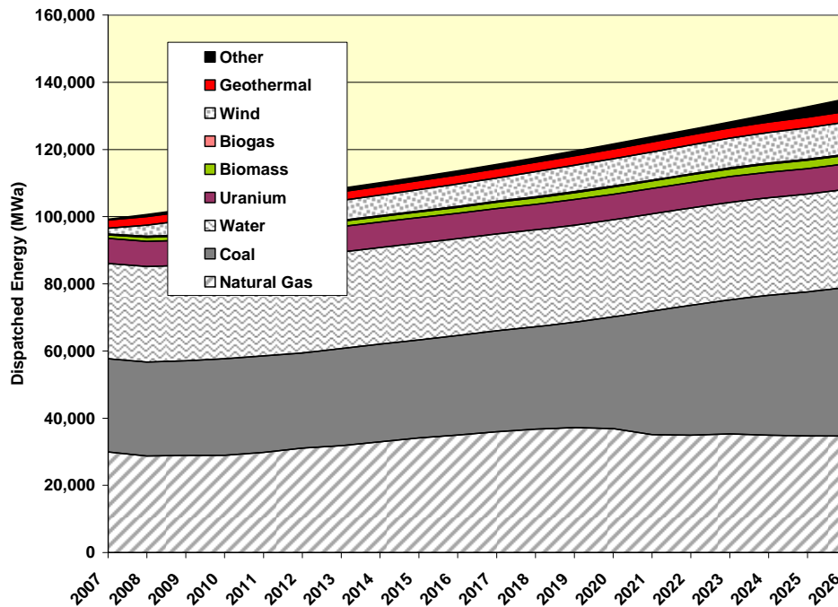
Figure 8: Forecast WECC resource mix based on dispatched energy
