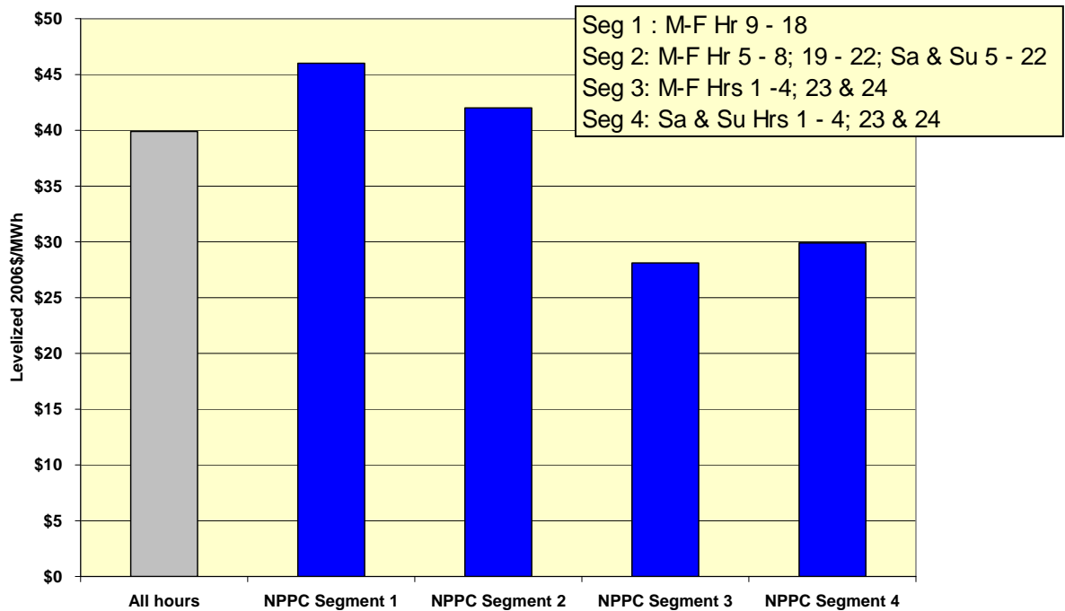
Figure 6: Forecast Mid-Columbia levelized energy prices by load segment
