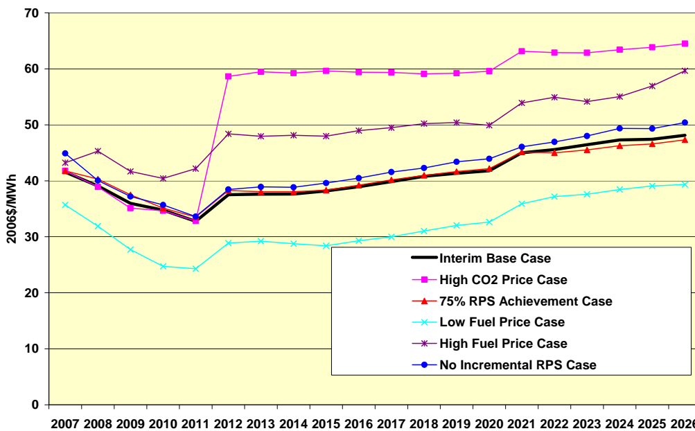
Figure 13: Interim base case and sensitivity case wholesale power price forecasts
